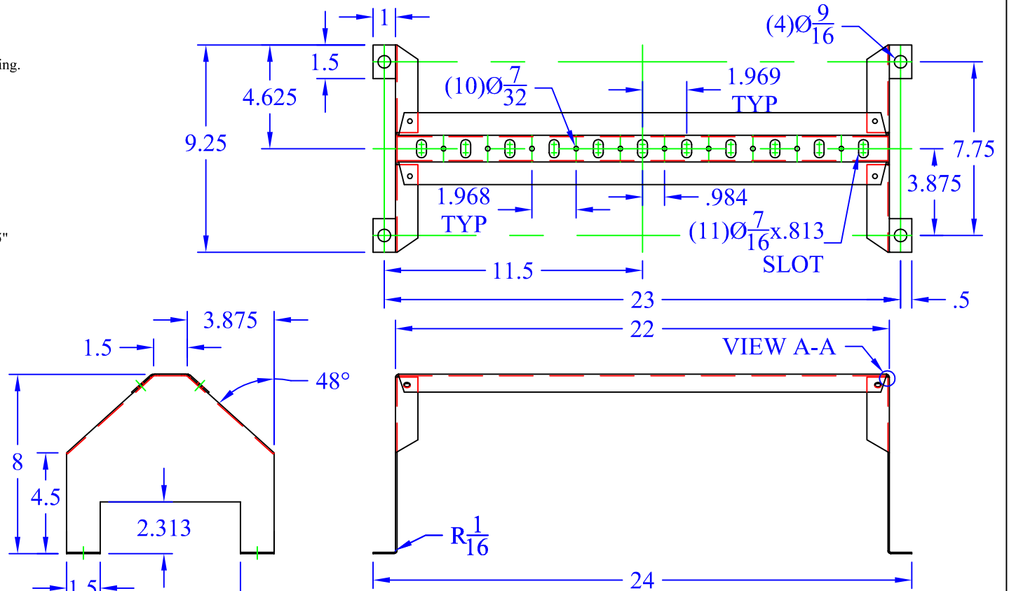
UNDER FLOOR SUPPORT SCALE: 2"=1'
