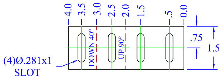
Flat Layout Plan View
