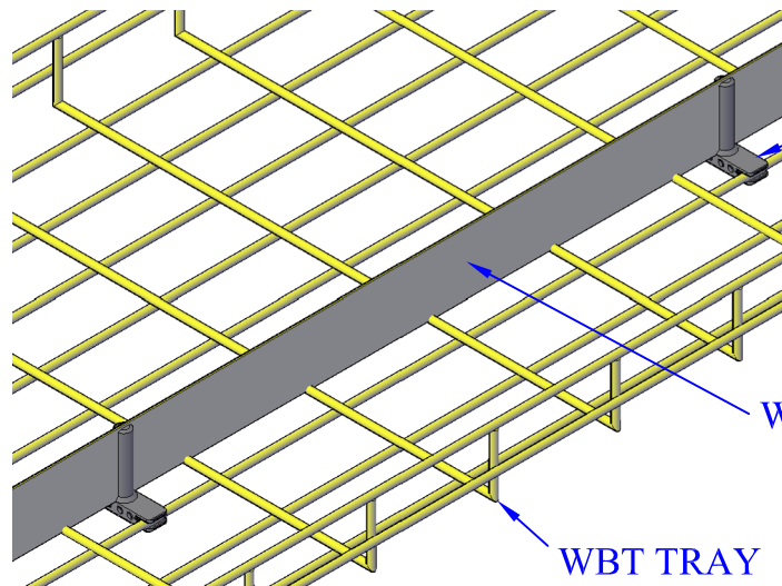
2" Divider Layout
