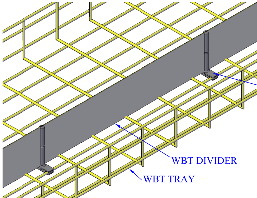
4" & 6" Divider Layout
