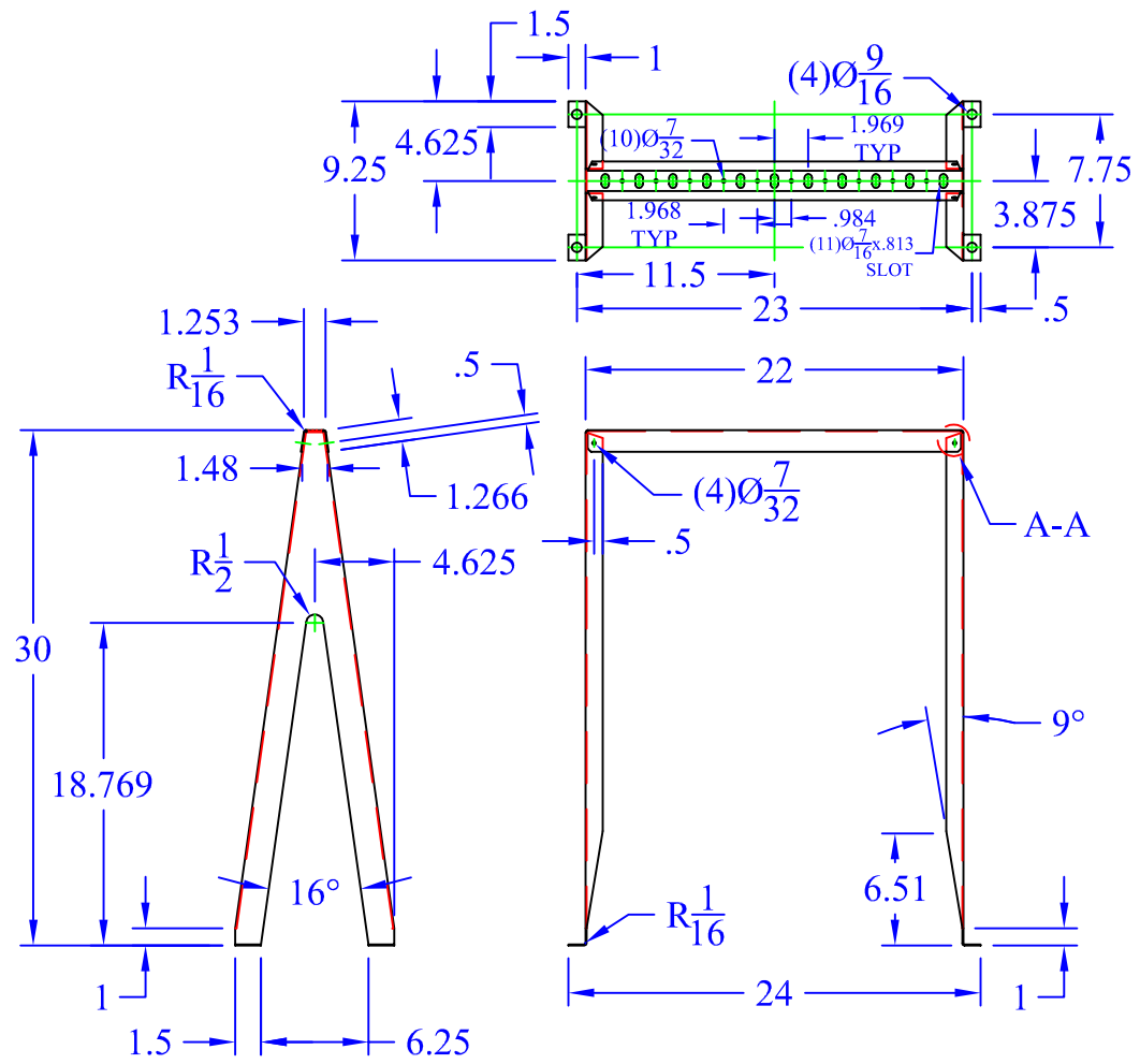
FLOOR SUPPORT SCALE: 1"=1'
