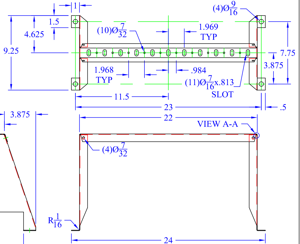
FLOOR SUPPORT SCALE:2"=1'
