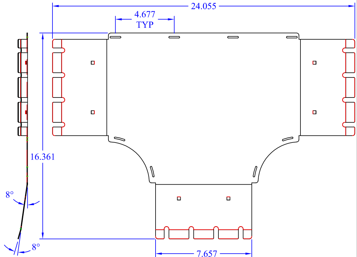
(1) WBT-T-Xx8 BASE
