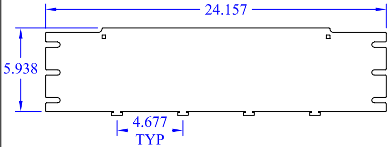
(1) WBT-T-6x8 TBACK
