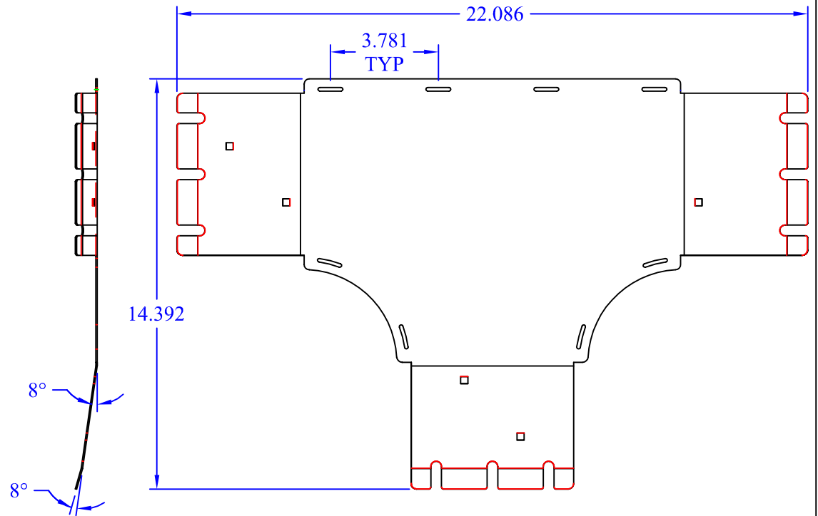
(1) WBT-T-Xx6 BASE
