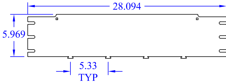
(1) WBT-T-6x12 TBACK
