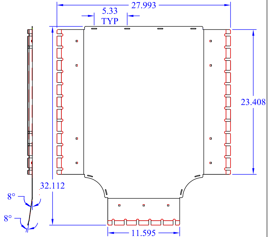
(1) WBT-T-Xx24-18PG BASE
