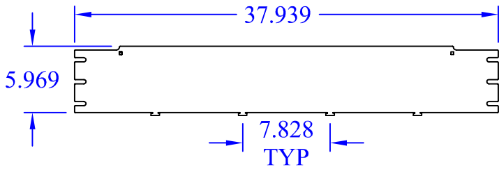
(1) WBT-T-6x22 TBACK
