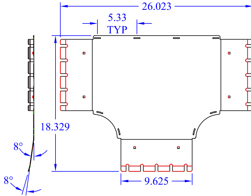
(1) WBT-T-Xx10 BASE
