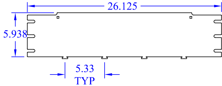
(1) WBT-T-6x10 TBACK
