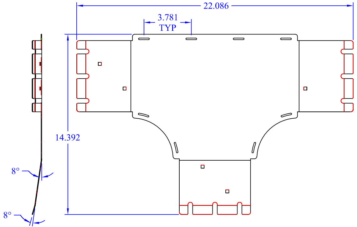
(1) WBT-T-Xx6 BASE
