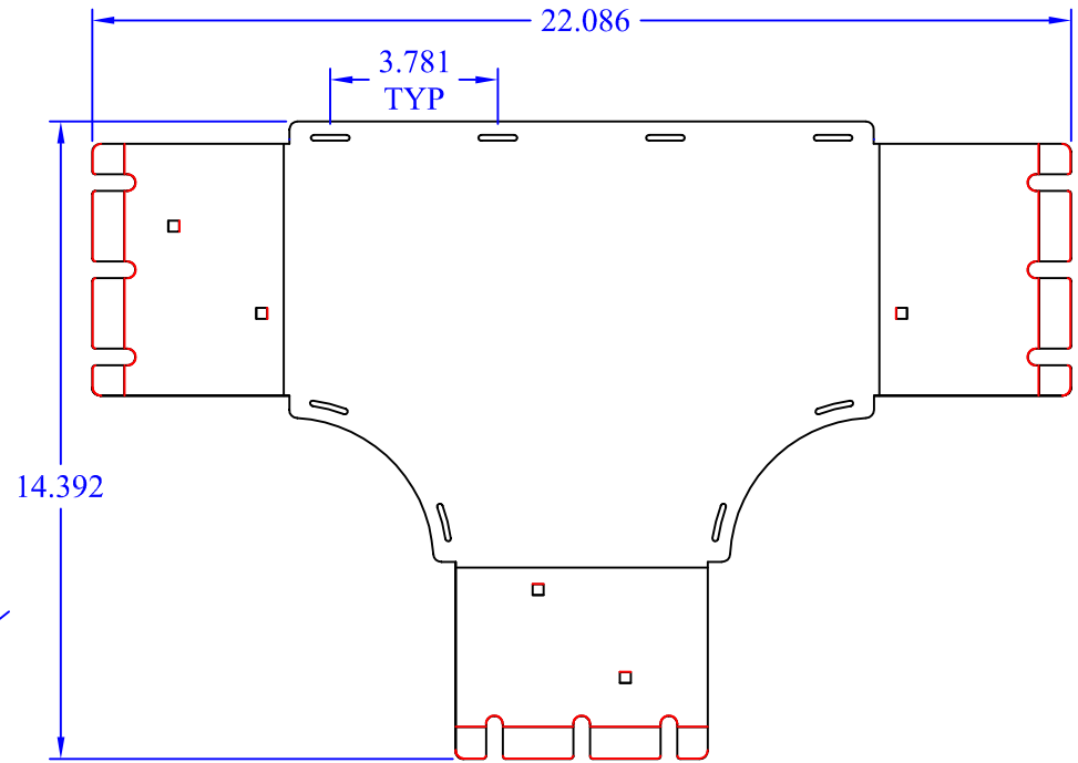
(1) WBT-T-Xx6 BASE
