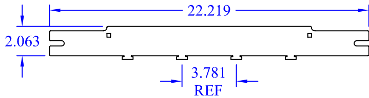
(1) WBT-T-2x6 TBACK
