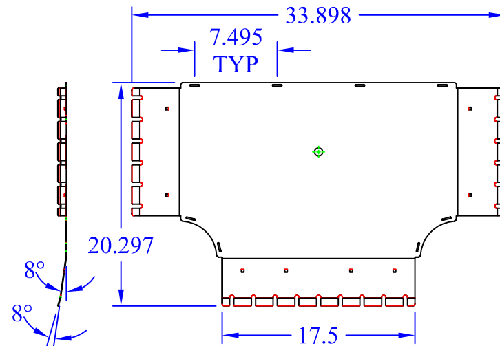
(1) WBT-T-Xx18 BASE
