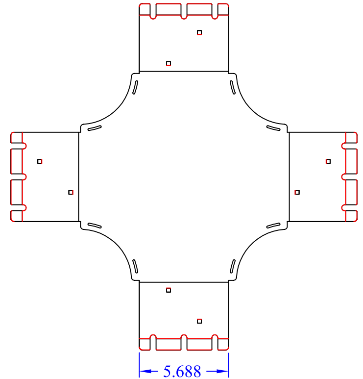
(1) WBT-I-Xx6 Base
