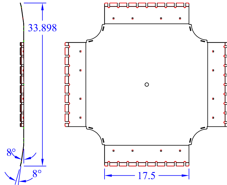
(1) WBT-I-Xx18 Base
