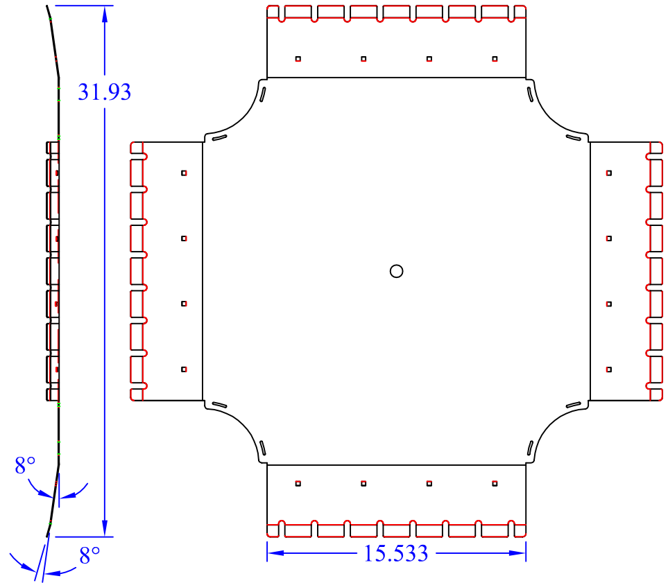
(1) WBT-I-Xx16 Base
