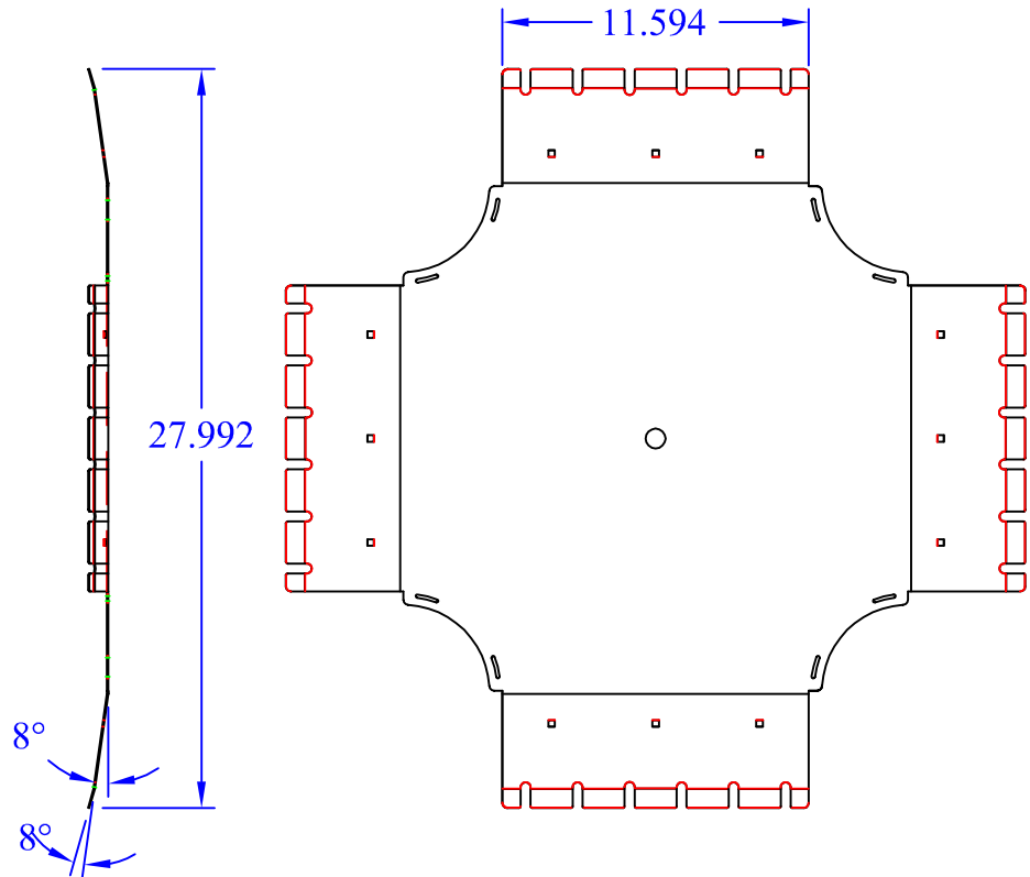
(1) WBT-I-Xx12 Base
