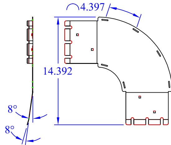
(1) WBT-90-Xx6 Base
