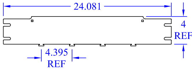
(1) WBT-90-4x6 OR
