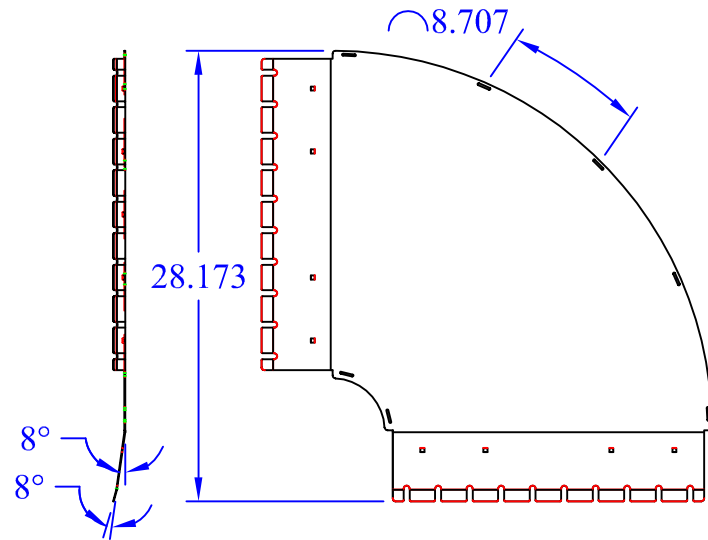
(1) WBT-90-Xx20 Base
