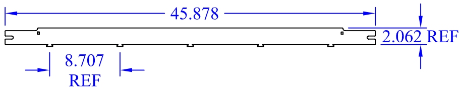
(1) WBT-90-2x20 OR
