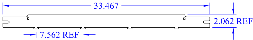
(1) WBT-90-2x12 OR
