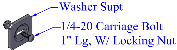
(4) Washer Supt
