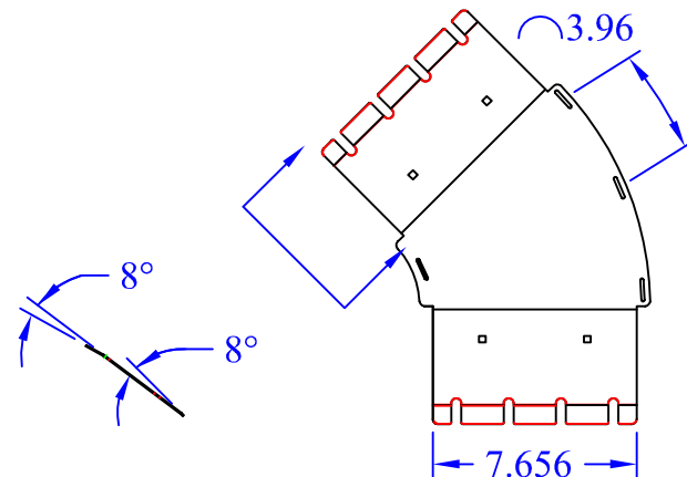
(1) WBT-45-Xx8 Base
