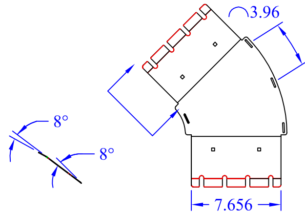
(1) WBT-45-Xx8 Base
