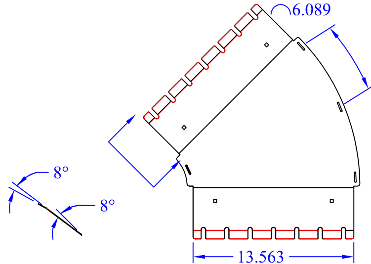
(1) WBT-45-Xx14 Base
