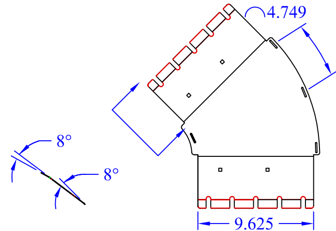
(1) WBT-45-Xx10 Base
