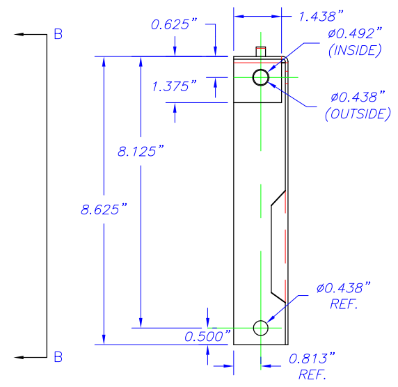
DETAIL B-B
