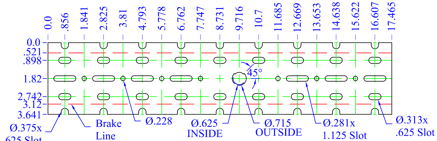
Flat Pattern Layout
