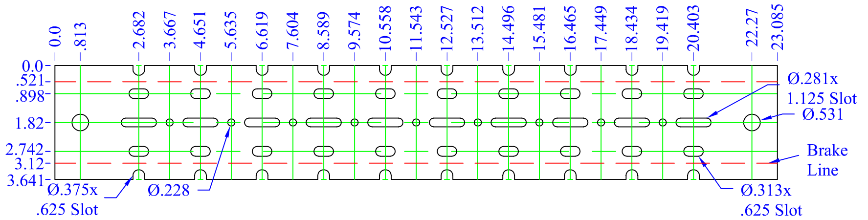
Flat Pattern View
