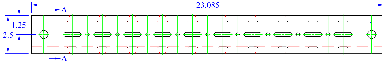
Formed View
