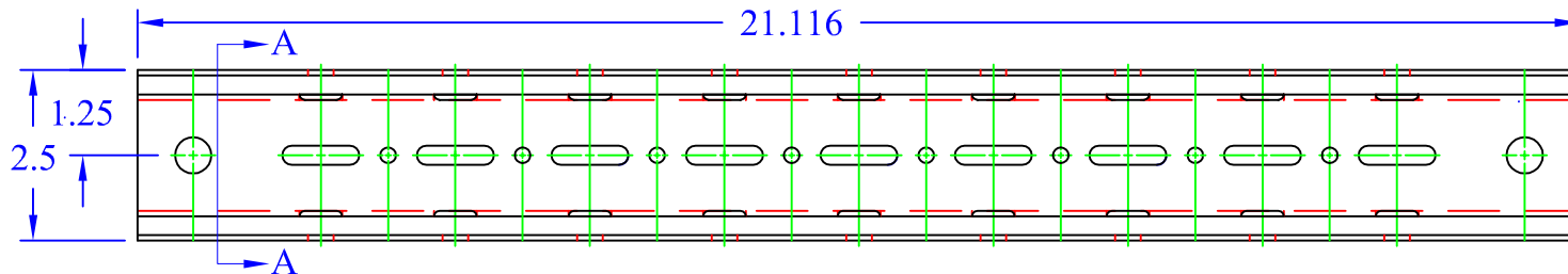
Formed View
