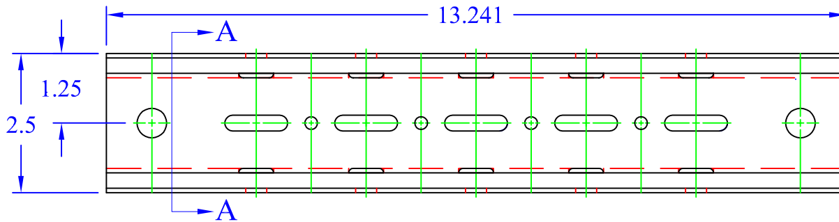
Formed View
