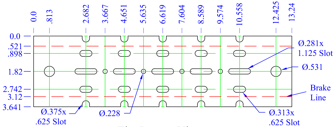
Flat Pattern View
