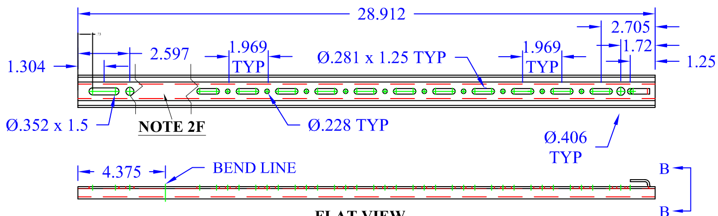
FLAT VIEW
