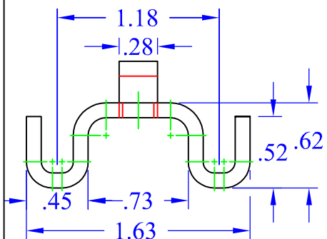
VIEW B-B 1:1 SCALE
