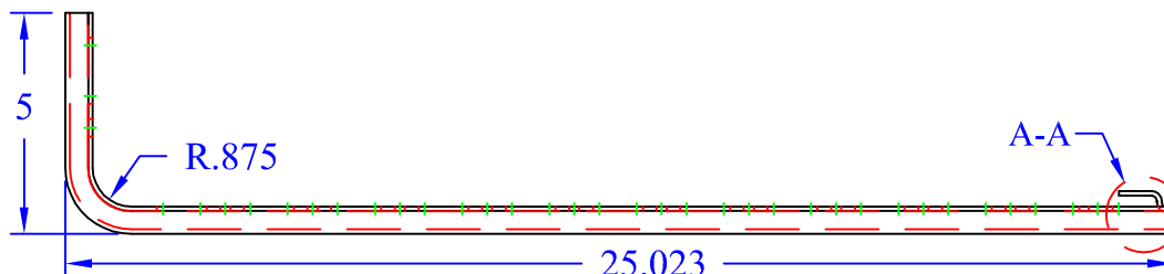
BENT VIEW
