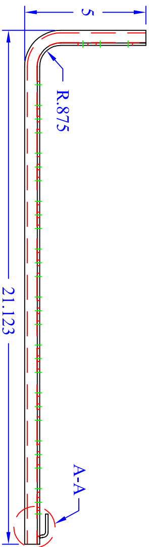
BENT VIEW
