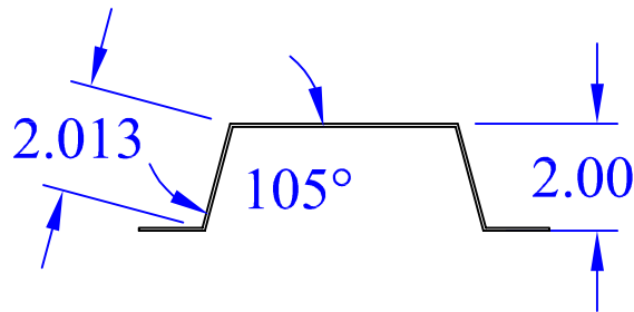
BENT VIEW
