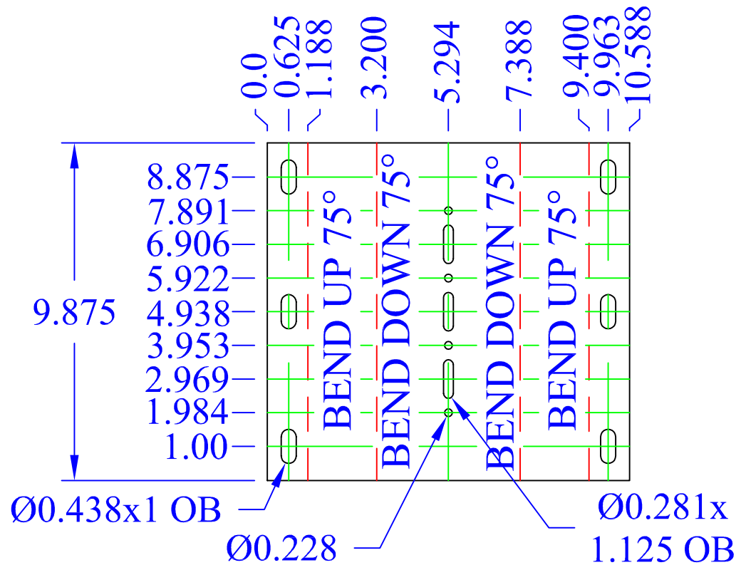
FLAT LAYOUT PLAN
