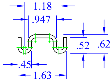
VIEW A-A 6"=1'
