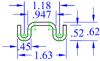
VIEW A-A 6"=1'
