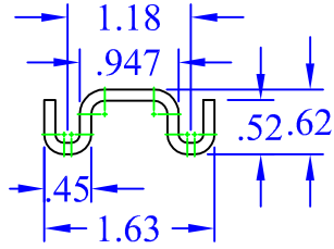
VIEW A-A 6"=1'
