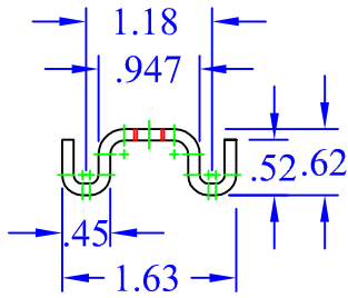
VIEW A-A 6"=1'
