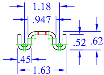
VIEW A-A 6"=1'
