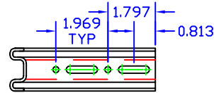
View B:B
